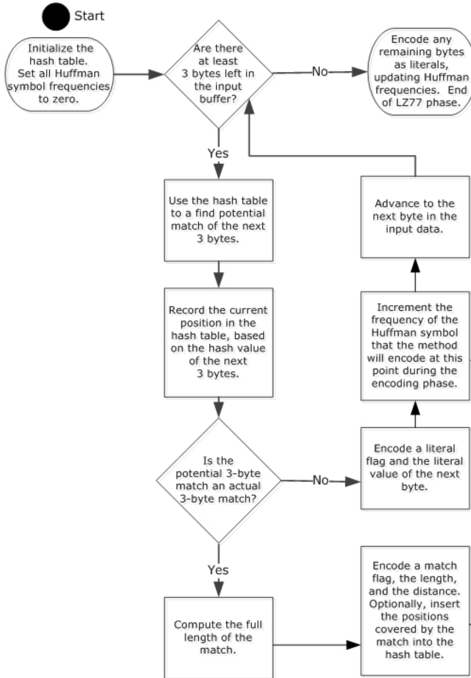
Figure 1: LZ77 phase
