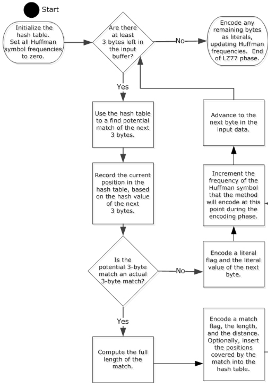
Figure 1: LZ77 phase
