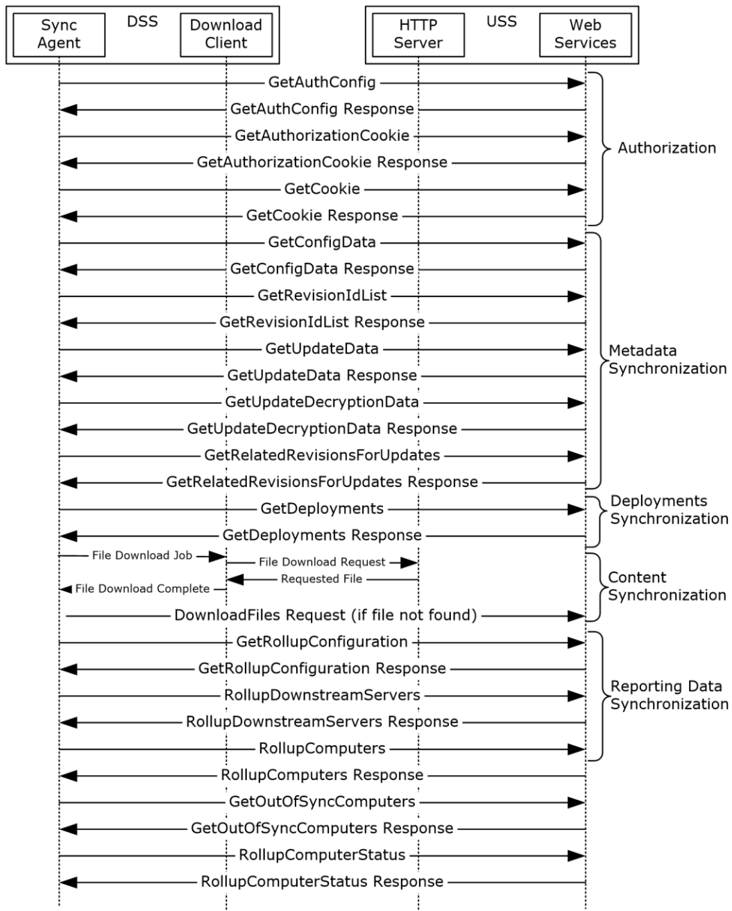
Figure 3: Message exchange
