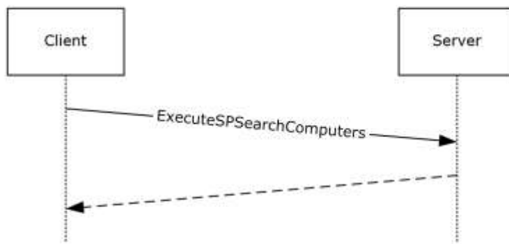
Figure 6: Searching for a client computer
