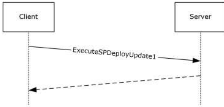
Figure 7: Creating the deployment
