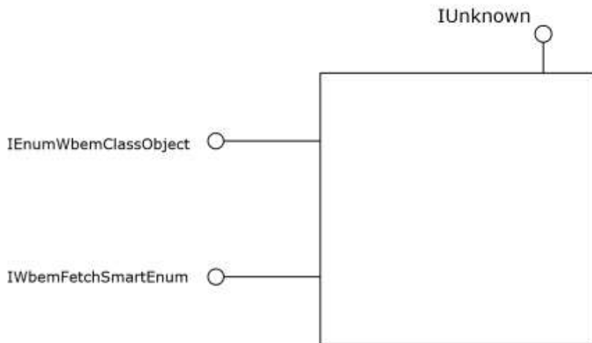
Figure 6: IEnumWbemClassObject interface
