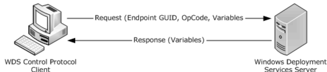
Figure 1: Client to server request
