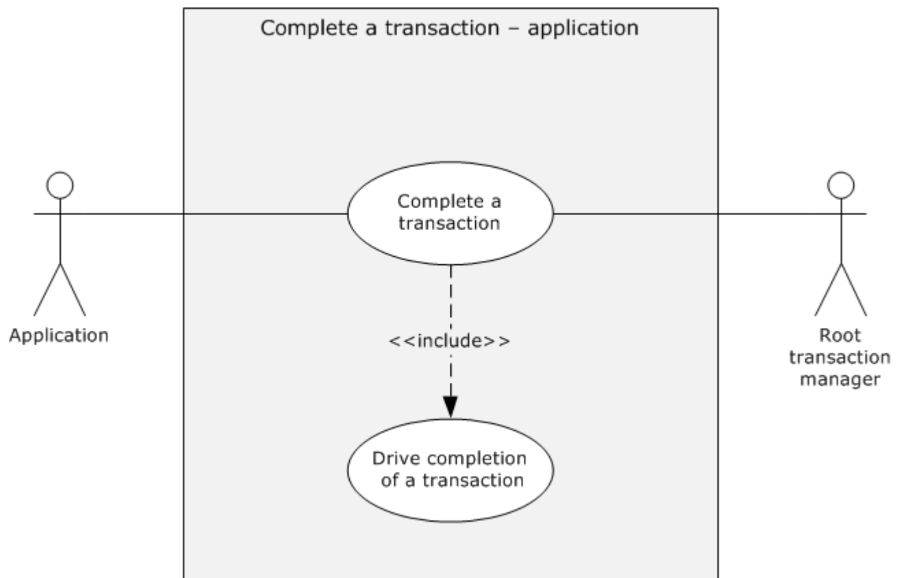
Figure 7: Use case diagram for transaction completion
