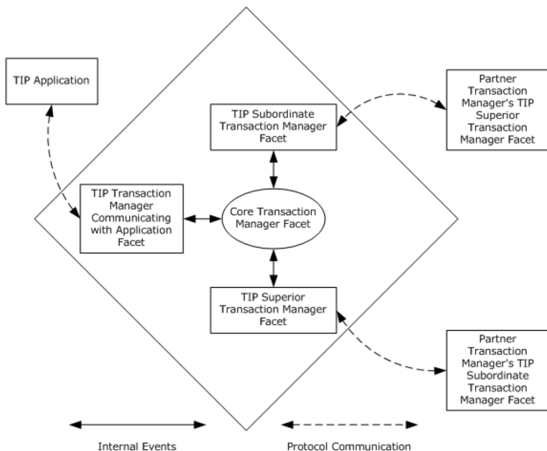
Figure 1: Protocol roles
