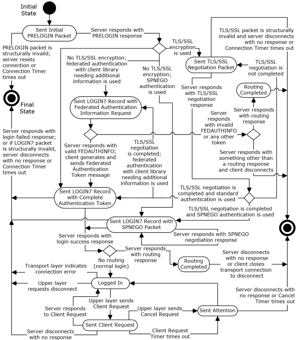
Figure 8: TDS client state machine
