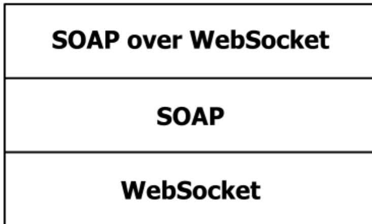
Figure 1: Protocol stack
