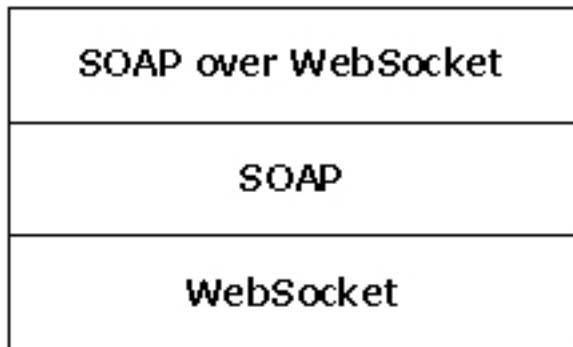
Figure 1: Protocol stack
