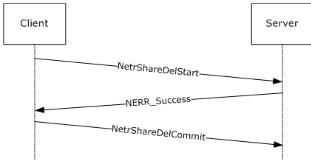
Figure 2: Two-phase share deletion
