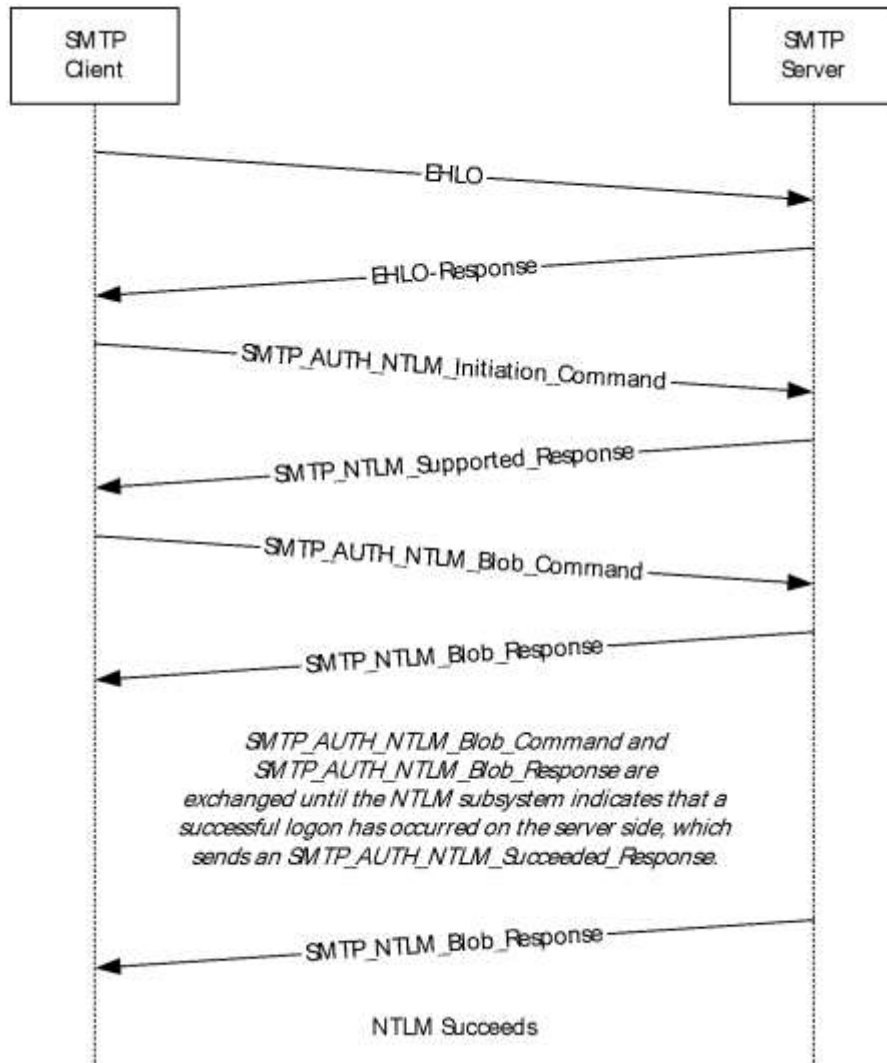
Figure 4: SMTP client successfully authenticating to SMTP server
