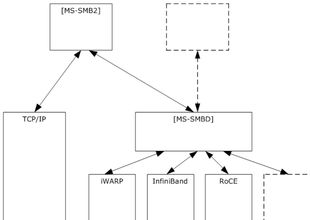
Figure 2: Protocol relationships
