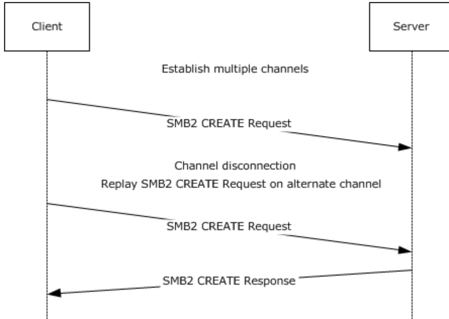
Figure 14: Replay Create Request on an alternate channel
