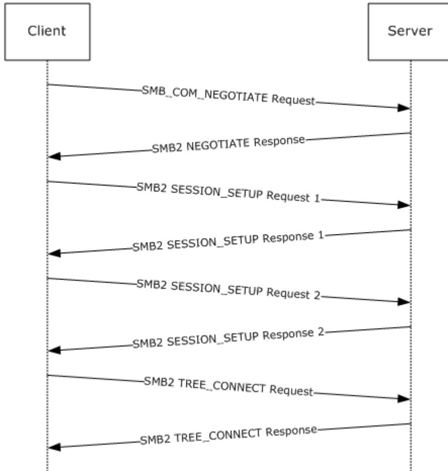
Figure 6: Client negotiating SMB2 with SMB-style negotiate
