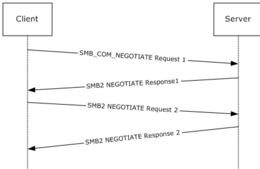
Figure 7: Client negotiating SMB 2.10 dialect with SMB-style negotiate
