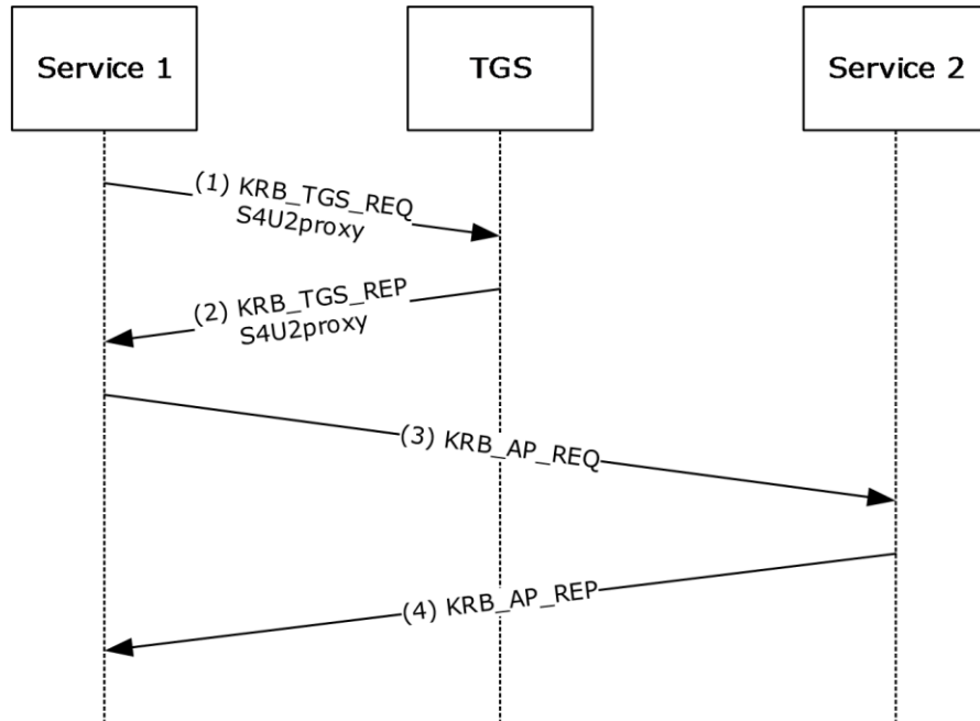
Figure 6: S4U2proxy Example
