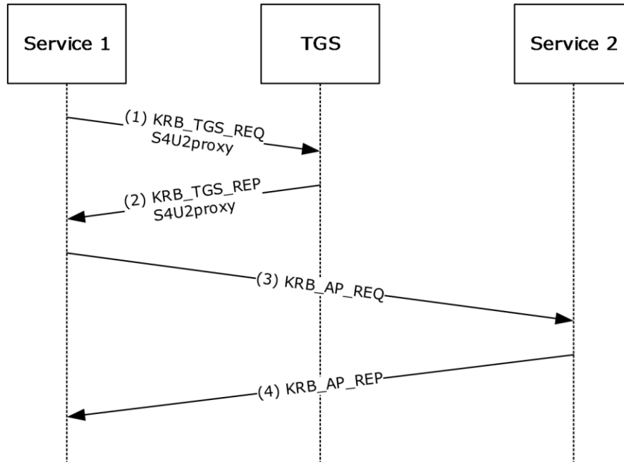
Figure 6: S4U2proxy Example
