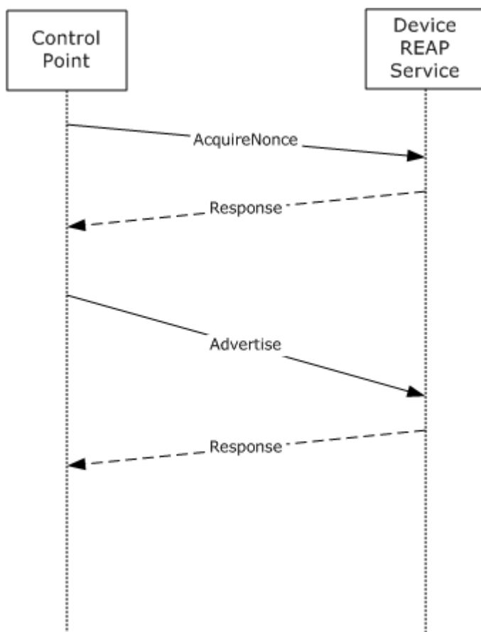
Figure 1: Protocol message sequence diagram (Advertise action)
