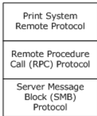
Figure 4: Protocol Relationships
