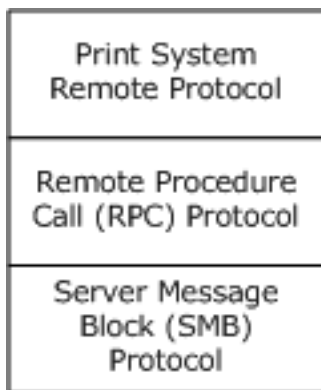
Figure 4: Protocol Relationships
