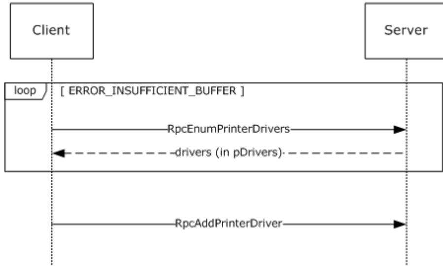
Figure 6: Adding a printer driver to a server
