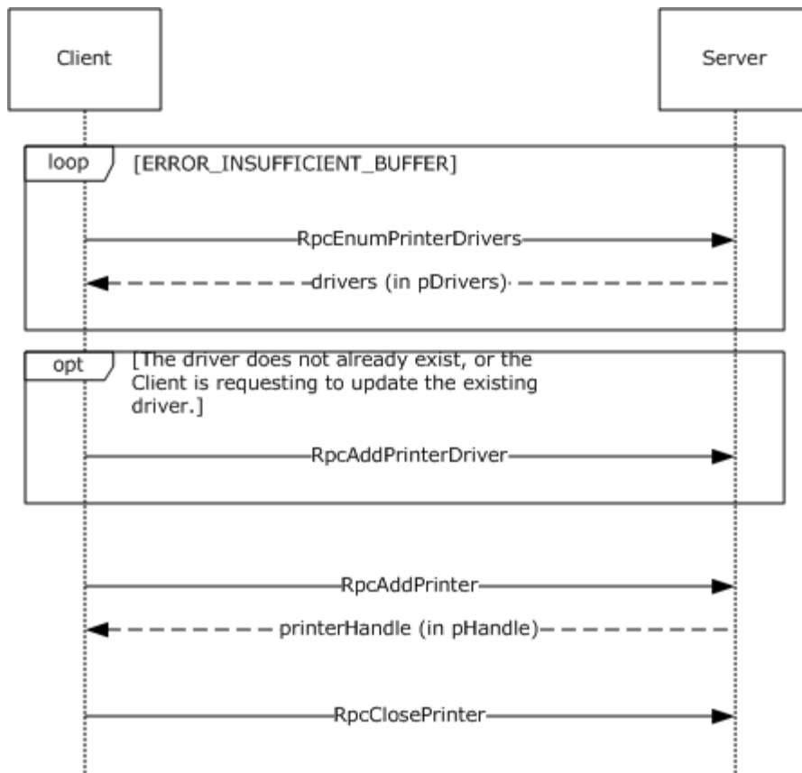
Figure 5: Adding a printer to a server
