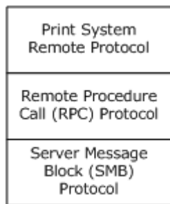
Figure 4: Protocol Relationships
