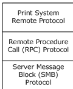
Figure 4: Protocol Relationships
