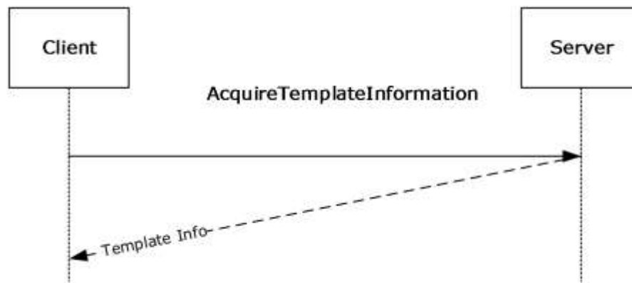
Figure 9: AcquireTemplateInformation sequence
