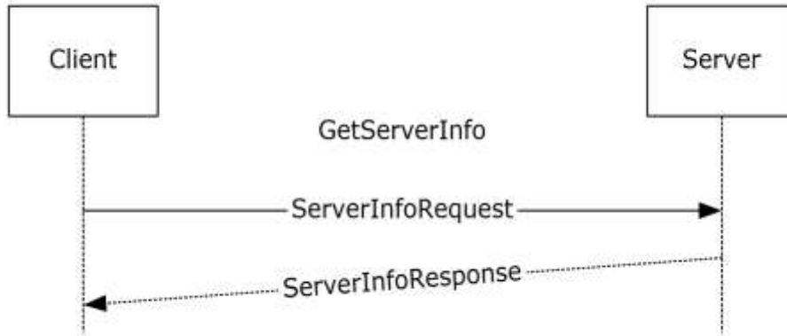
Figure 16: GetServerInfo sequence
