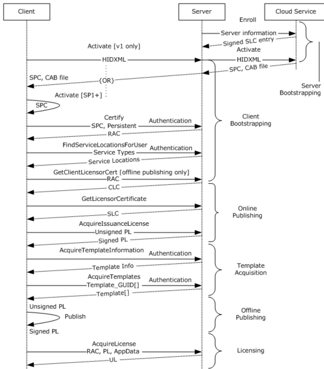
Figure 5: Protocol operation
