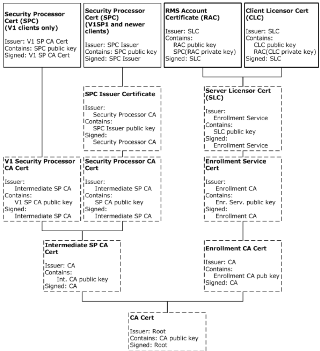
Figure 3: Relationships between certificates
