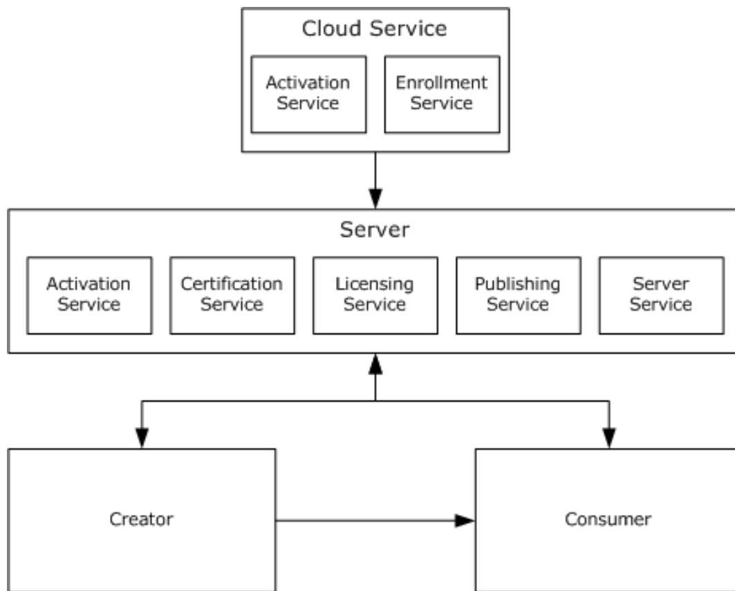
Figure 1: Rights management roles
