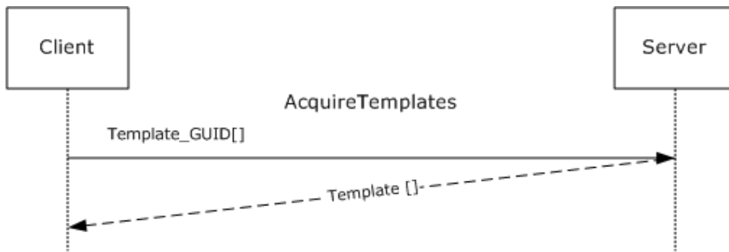
Figure 10: AcquireTemplates message sequence
