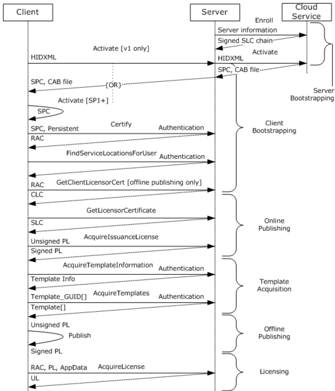
Figure 16: Common message sequence for the client
