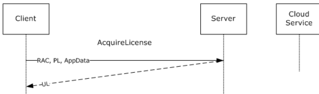
Figure 8: AcquireLicense message sequence
