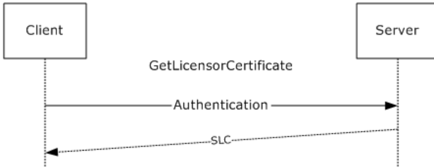
Figure 14: GetLicensorCertificate sequence
