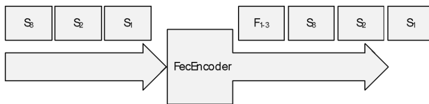
Figure 3: FEC engine
