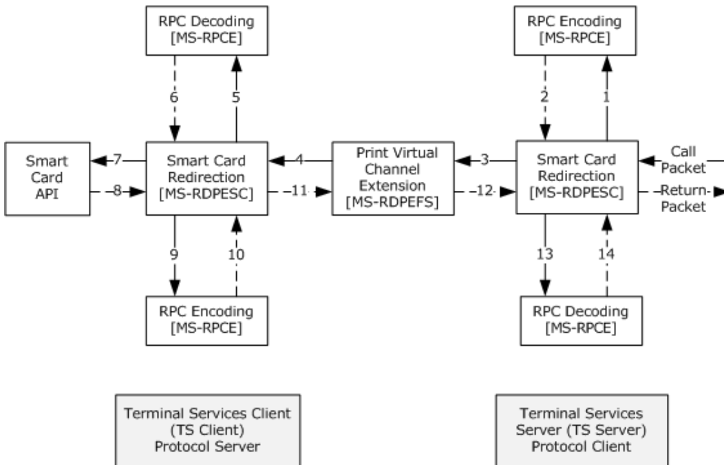
Figure 3: Protocol flow
