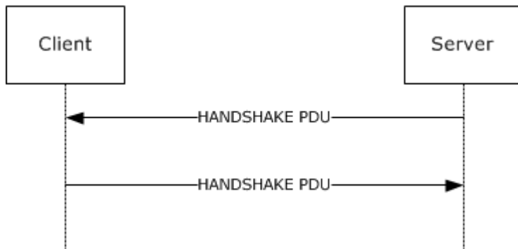
Figure 1: Handshake PDU
