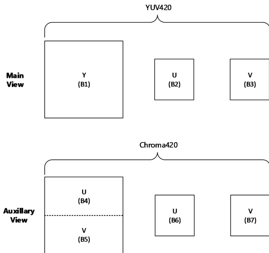
Figure 7: A representation of a YUV444 macroblock as two YUV420p macroblocks
