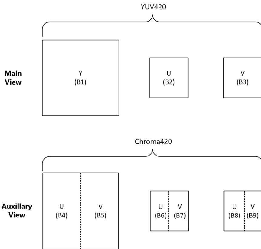
Figure 9: A representation of a YUV444 frame as two YUV420p frames
