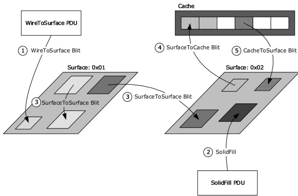
Figure 1: Overview of the blit commands
