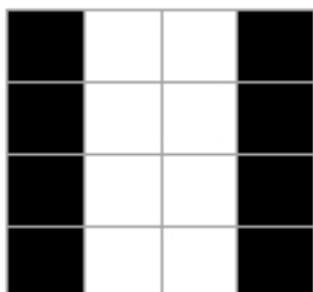
Figure 10: A 4 x 4 glyph
