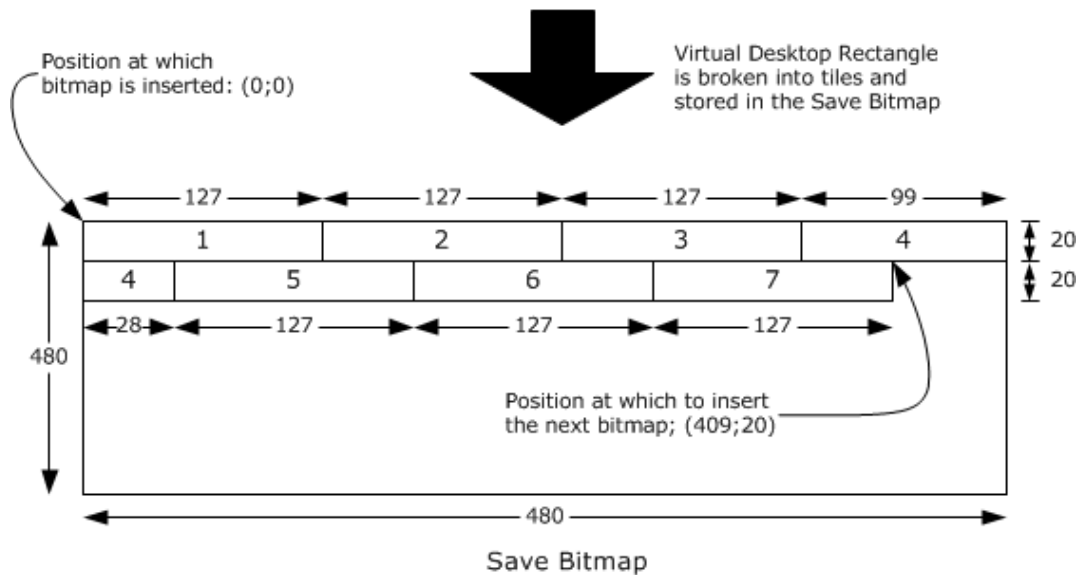
Figure 20: Illustration of Save Bitmap Primary Drawing Order
