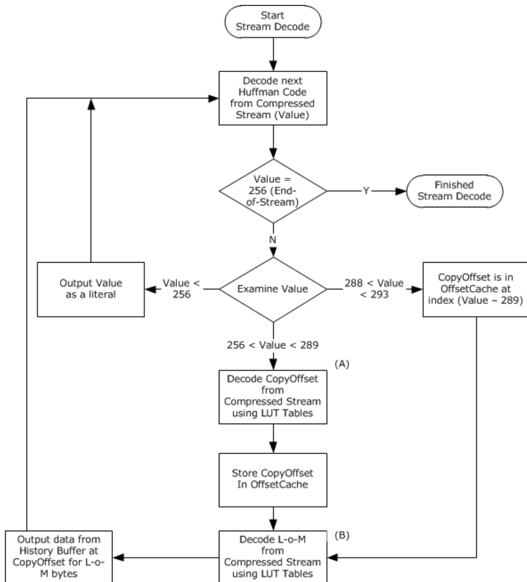
Figure 9: Decoding a compressed stream
