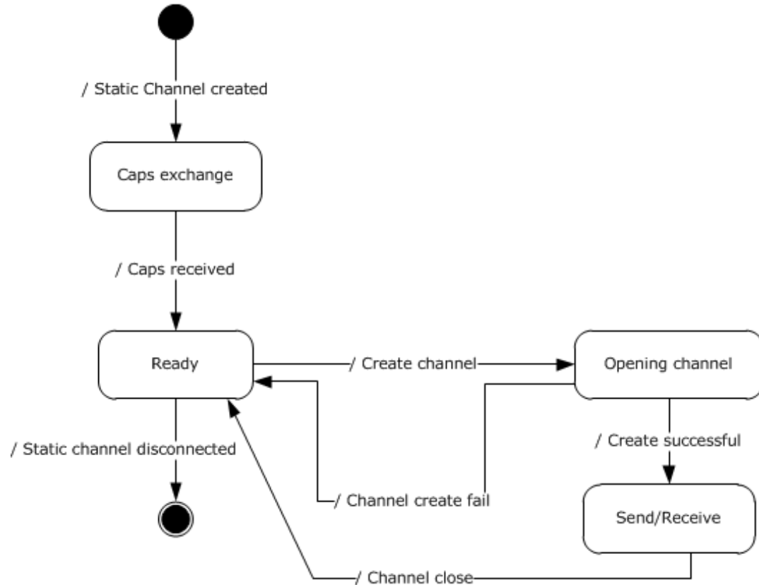
Figure 7: State diagram
