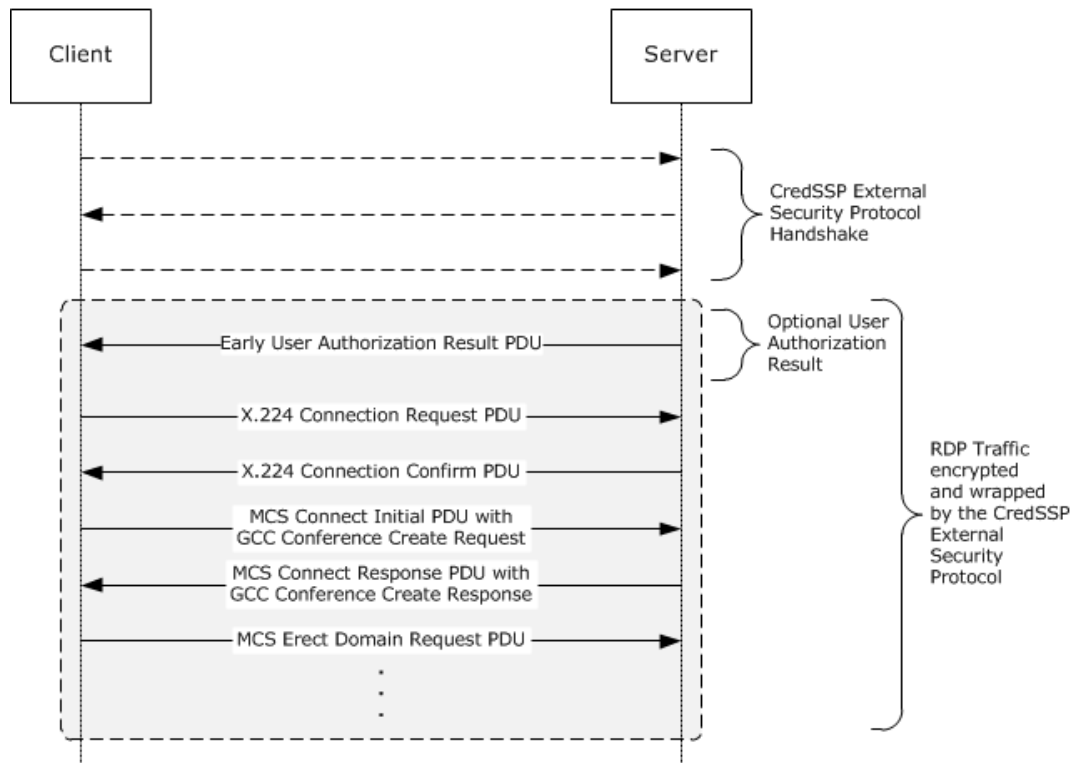
Figure 14: Direct security-enhanced connection sequence
