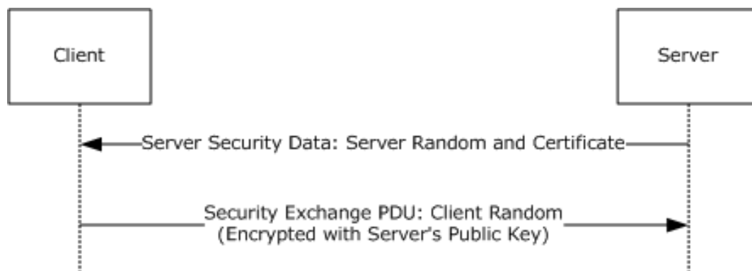
Figure 9: Client and server random value exchange
