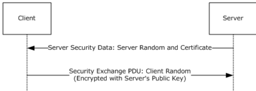
Figure 8: Client and server random value exchange
