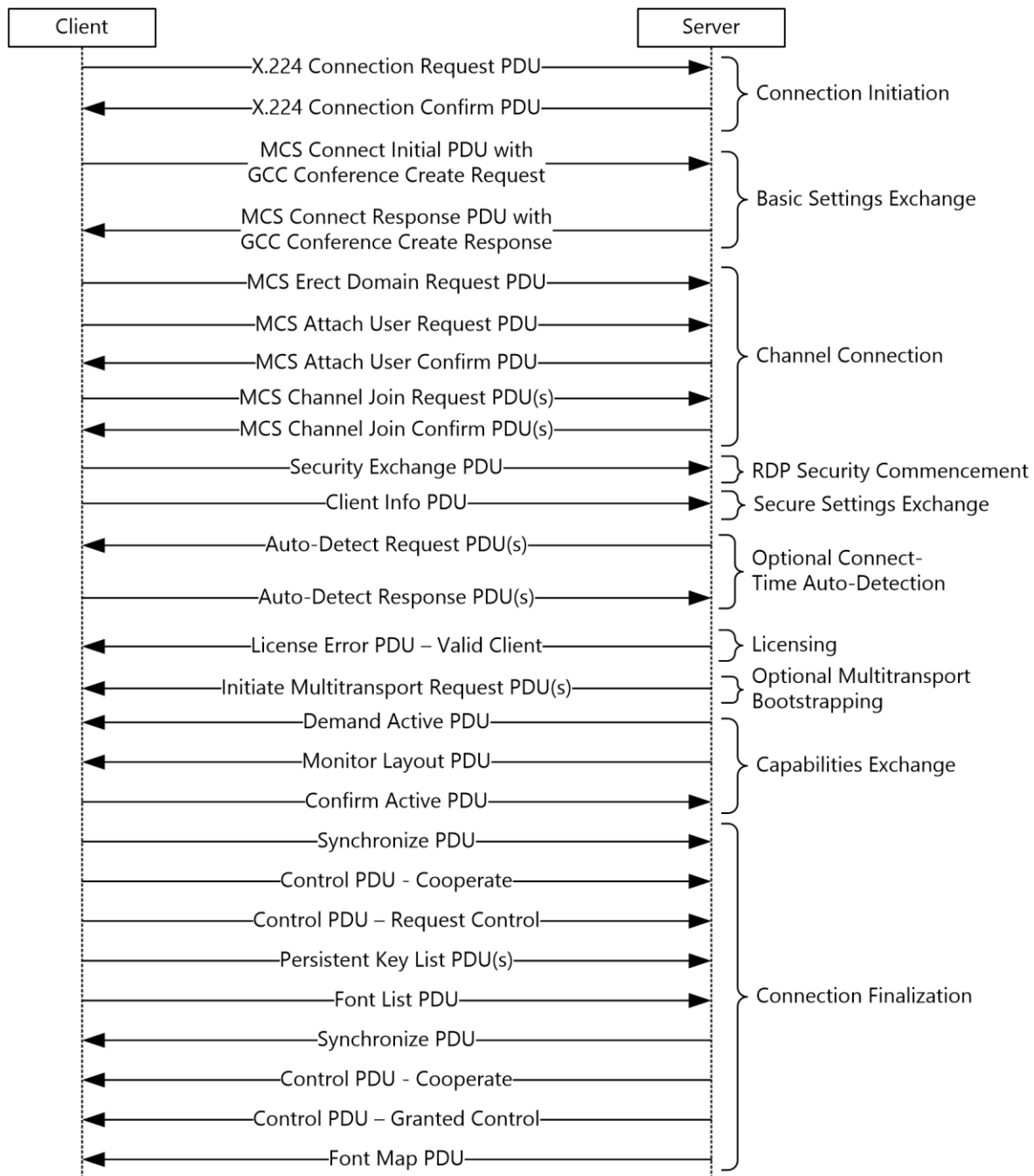
Figure 1: Remote Desktop Protocol (RDP) connection sequence
