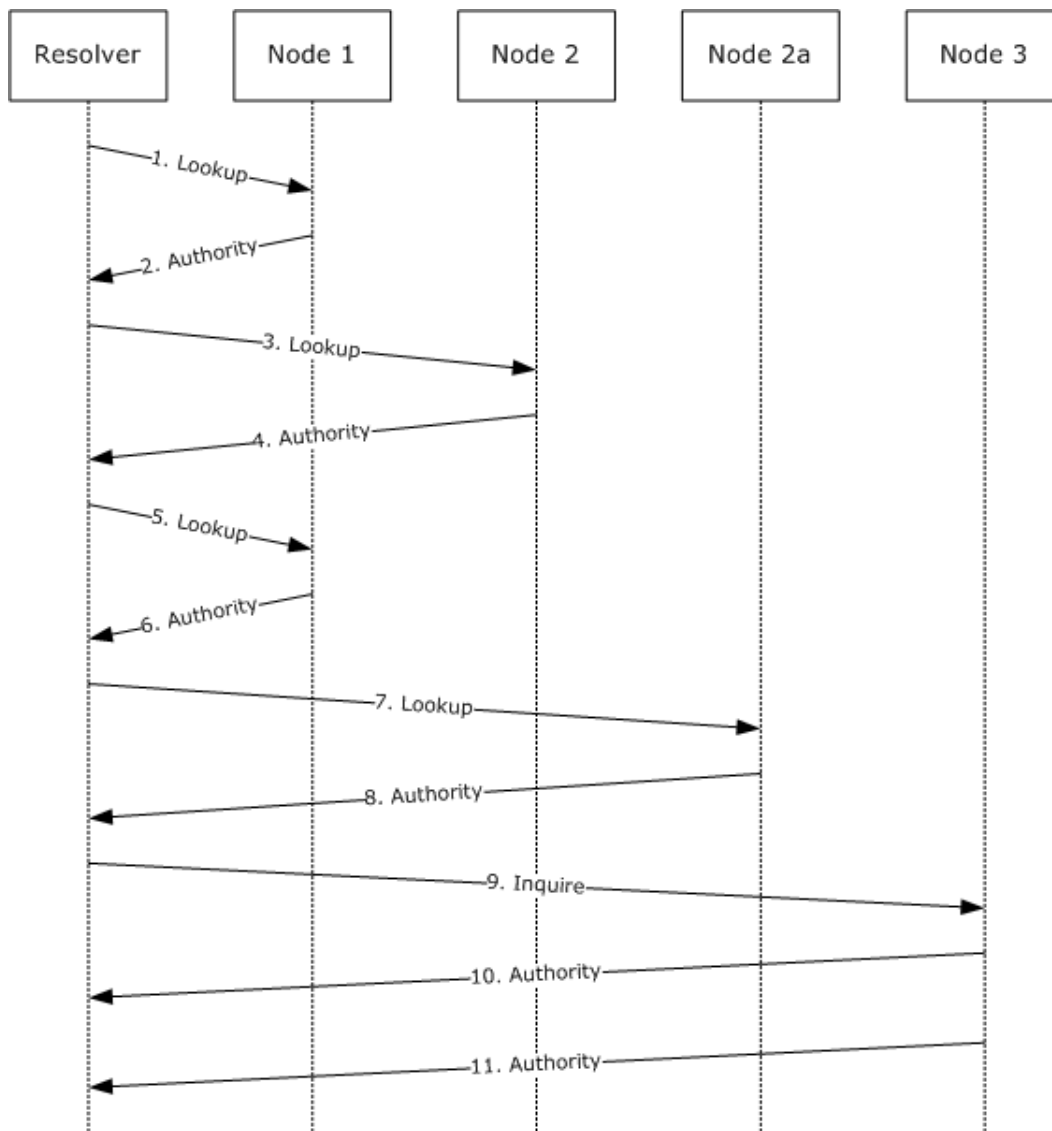
Figure 5: Peer Name resolution
