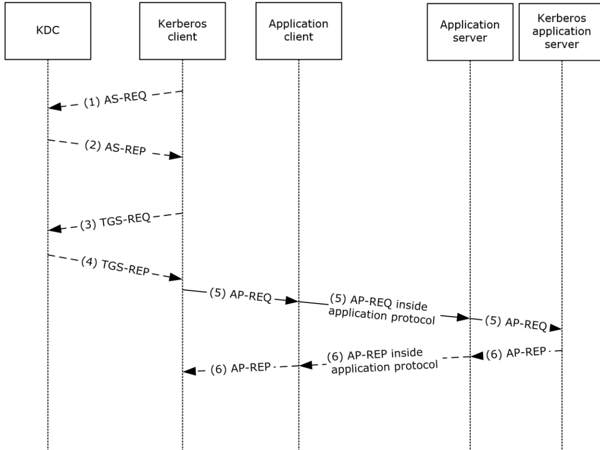
Figure 2: Network logon
