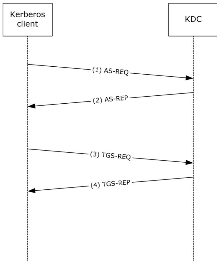
Figure 1: Interactive logon
