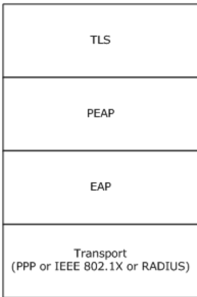
Figure 2: Protocol layering during phase 1 of PEAP
