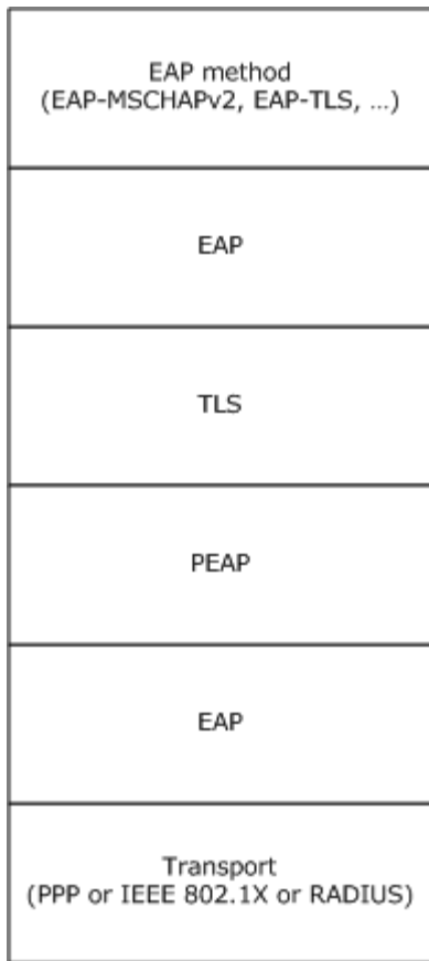
Figure 3: Protocol layering during phase 2 of PEAP
