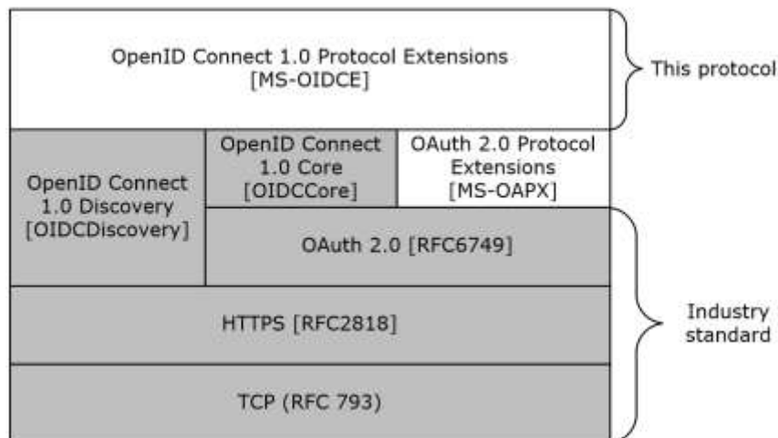
Figure 1: Protocol dependency
