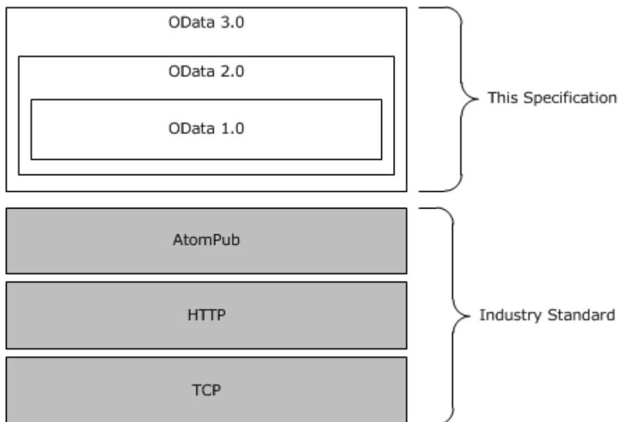
Figure 1: OData Relationship to Other Protocols
