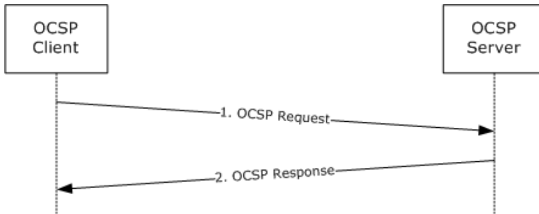
Figure 2: Revocation-checking process
