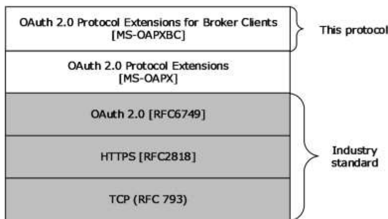
Figure 1: Protocol dependency
