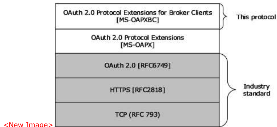
Figure 1: Protocol dependency
