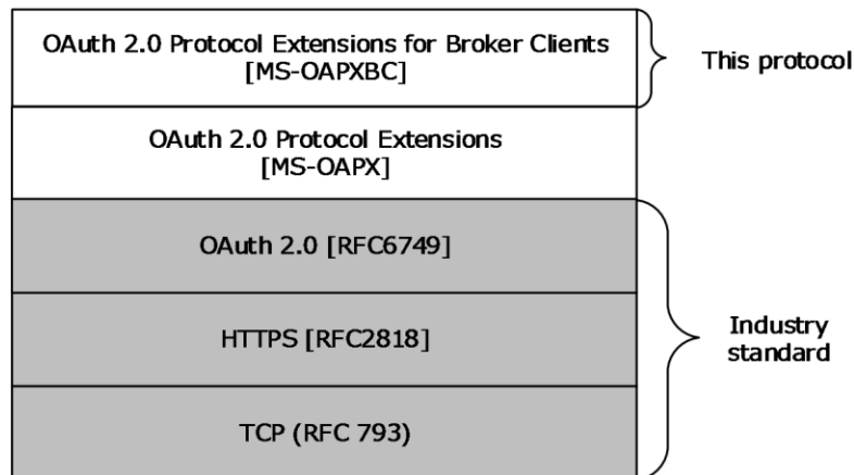
Figure 1: Protocol dependency
