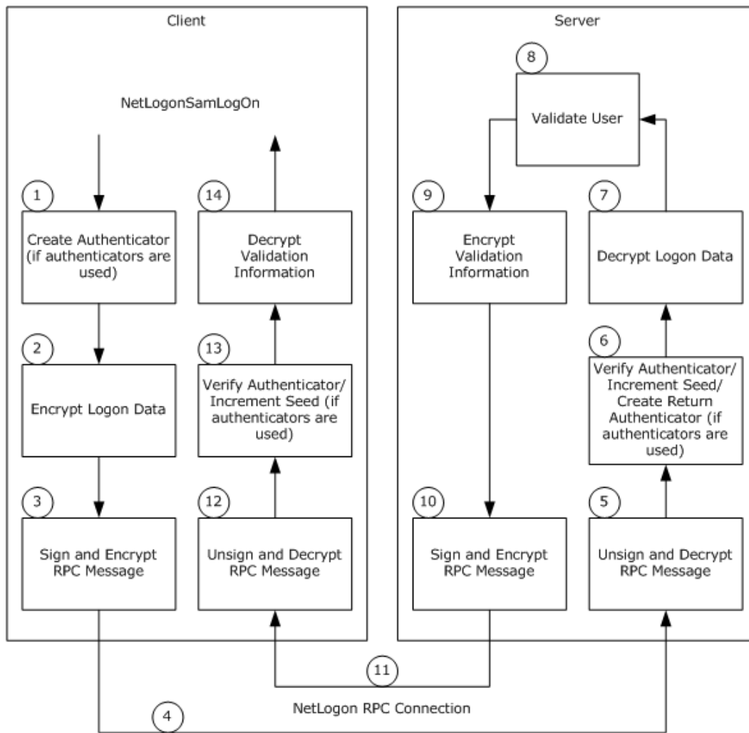
Figure 10: Secure channel execution of NetLogonSamLogon
